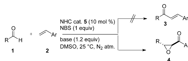
Scheme 1. NHC-catalyzed oxidative coupling of alkenes with aldehydes. DBU = 1,8-diazabicyclo [5.4. 0] undec-7-ene, DMSO = dimethylsulfoxide, NBS = N-bromosuccinimide.
